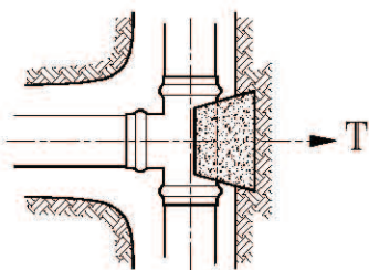
Tee anchorage
