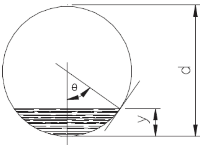
Figure 3.5 Angle of repose of sediment for a self-cleansing flow
