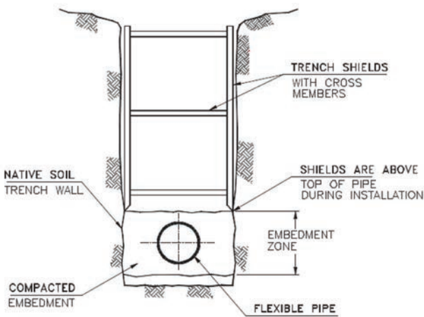
FIGURE 4.2 Shields kept above side support
