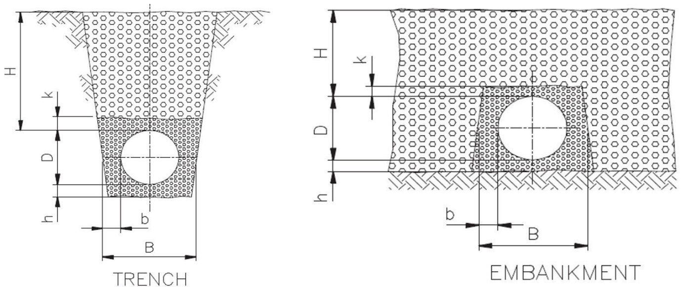
FIGURE 3.7 Critical dimensions for design and installation
