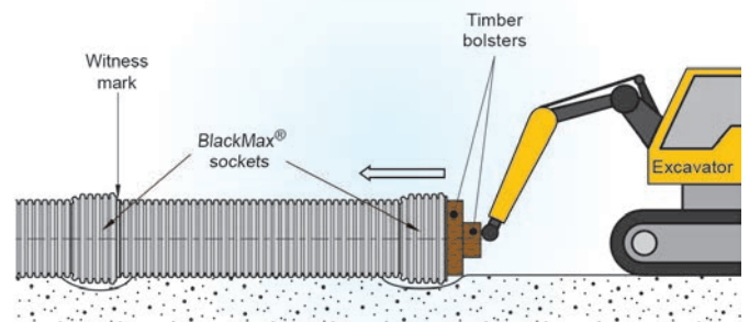
Larger pipes require mechanical force during the jointing procedure.
