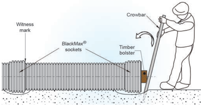
Generally smaller pipes can be pushed home with a crowbar.
